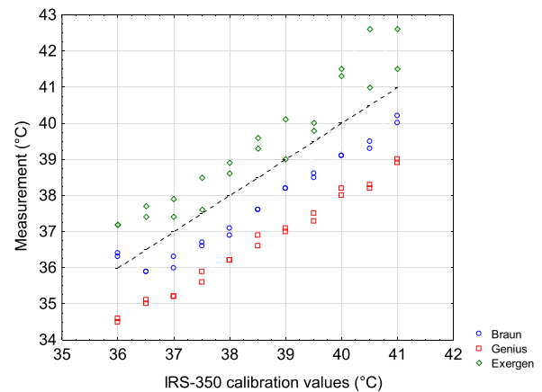
Figure 1. Calibration results: values from Voltcraft IRS-350 system on horizontal axis and values of two Braun Thermoscan® PRO 6000, Genius 3, and Exergen TAT-5000S-RS232 systems on vertical axis.
